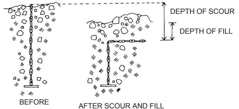
Figure 63. Scour chains and placement.
